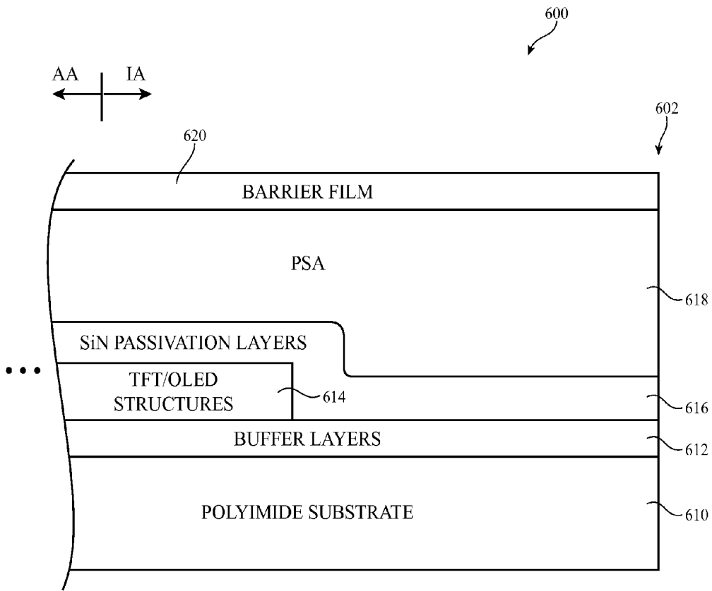
FIG. 6 (PRIOR ART)
